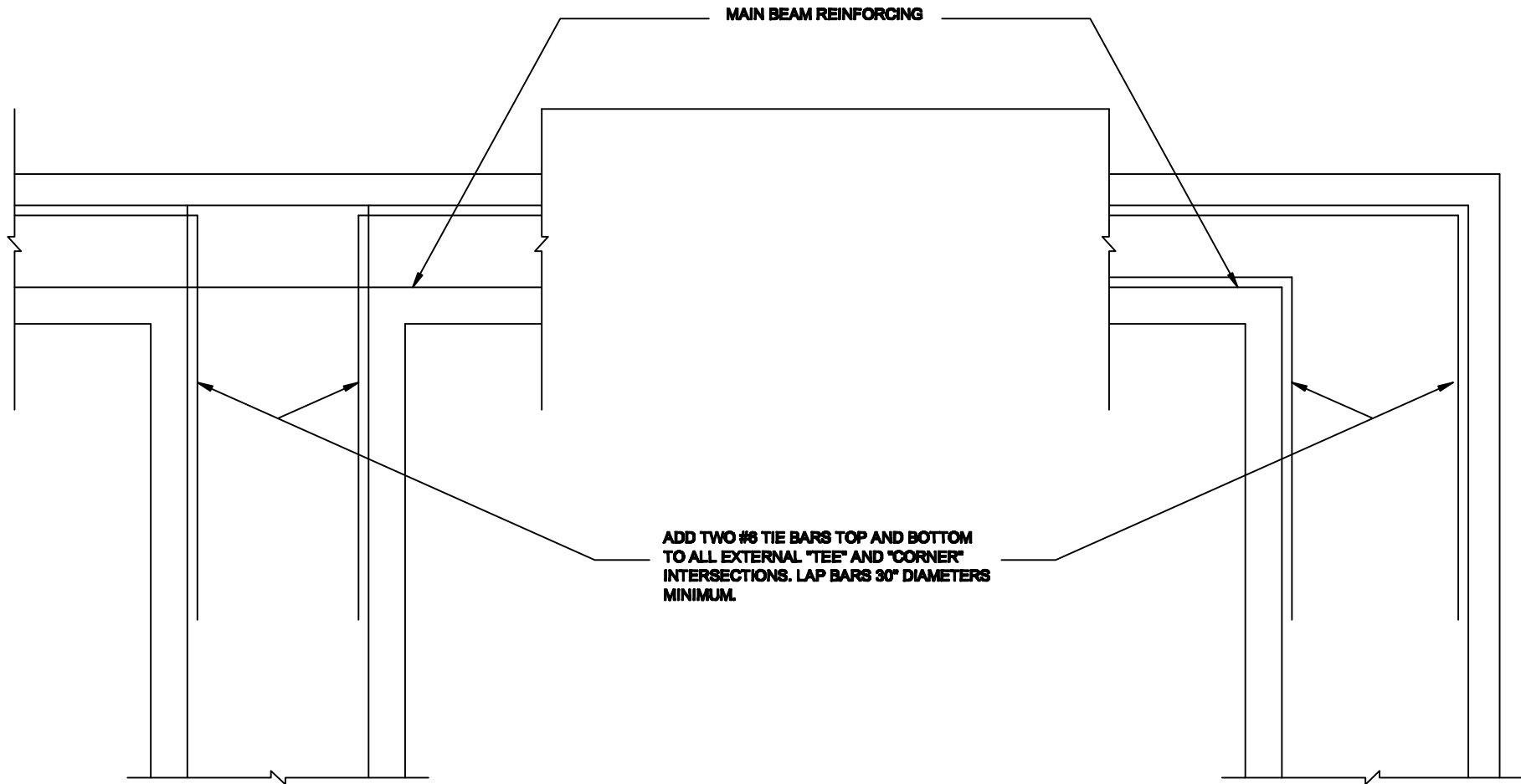
EXTERNAL "TEE"
